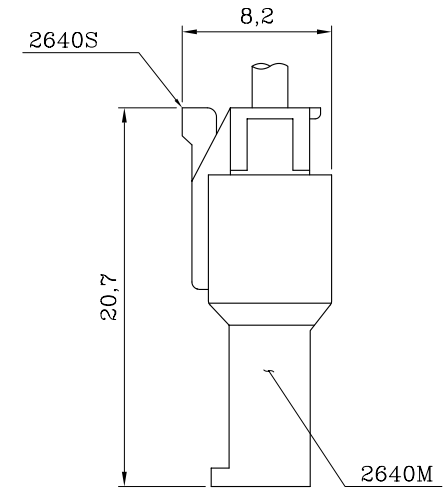
ASSEMBLY LAYOUT
