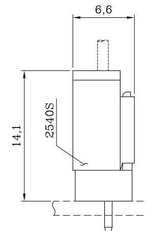
ASSEMBLY LAYOUT
