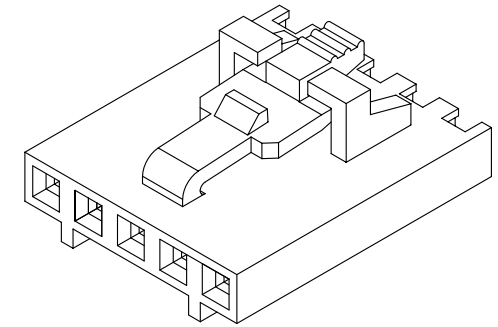
ISOMETRIC VIEW
