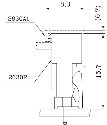
ASSEMBLY LAYOUT (WIRE-TO-BOARD)
