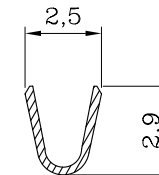
SEC. B-B'
