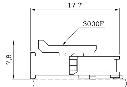
ASSEMBLY LAYOUT
