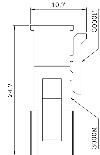
Assembly View
