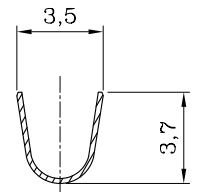
SEC. A-A'
