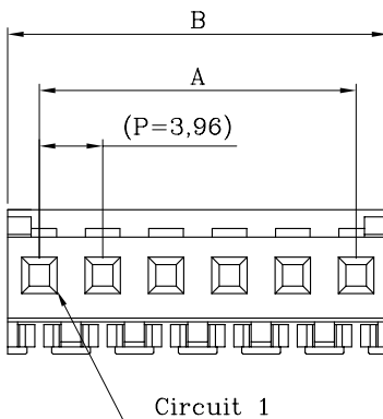
(Type - 2) With Ramp and Rib
