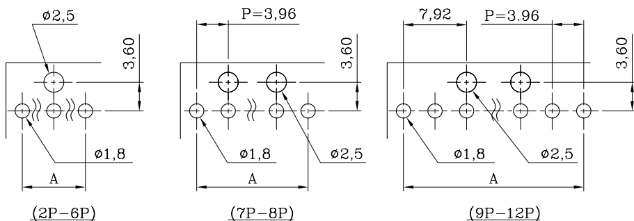
P.C. BOARD LAYOUT (COMPONENT SIDE)
