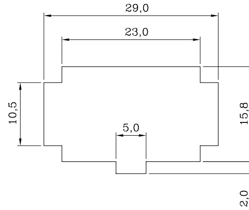
PANEL HOLE DIMENSION
