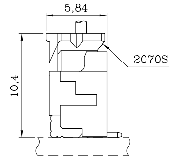
ASSEMBLY LAYOUT
