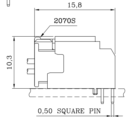
ASSEMBLY LAYOUT
