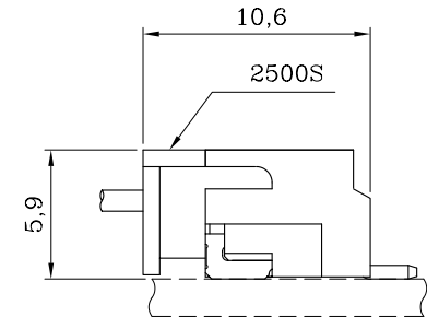
ASSEMBLY LAYOUT
